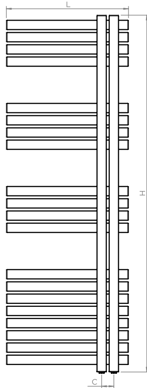
Front View
