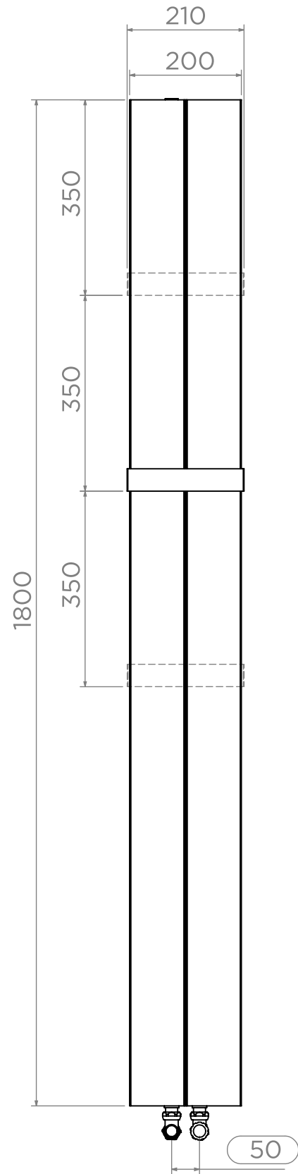
Front View
