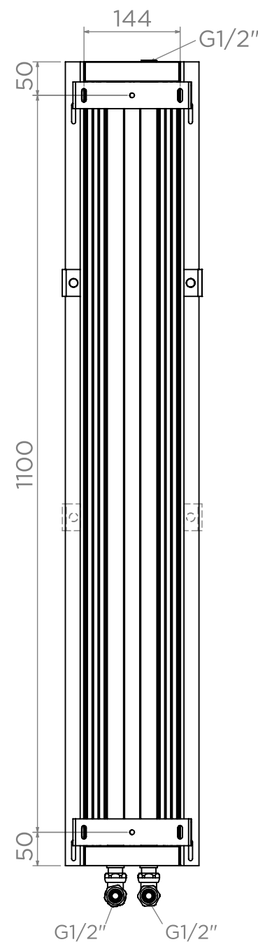
Back View
