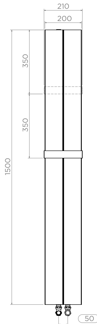
Side View
