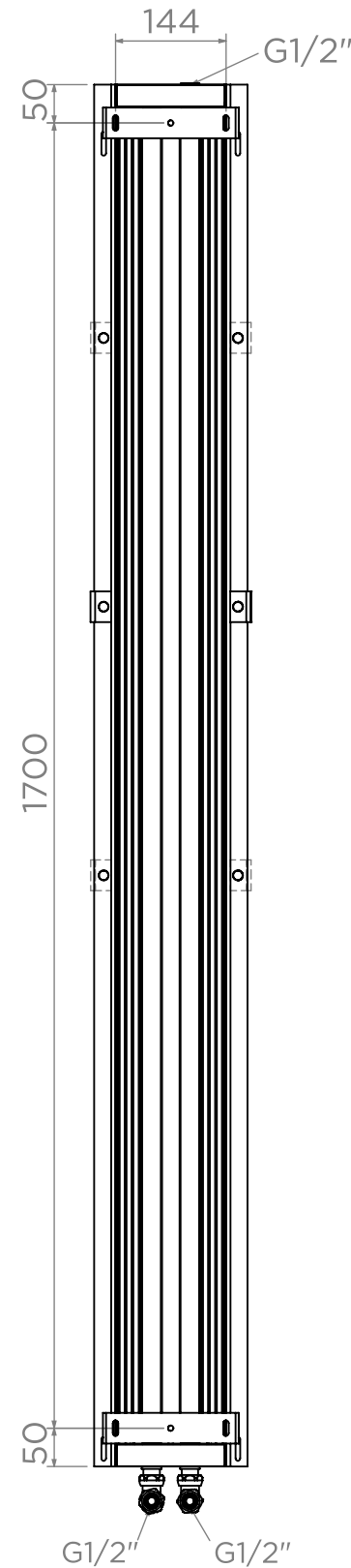
Back View
