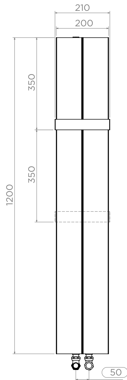
Front View
