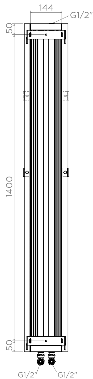
Front View
