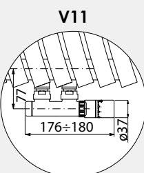
Measures for valves type Cordivari Elegant Square with thermostatic head and pipe centres 50 mm
