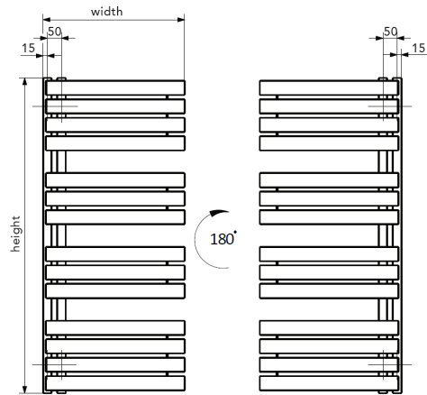
Bracket Positions
